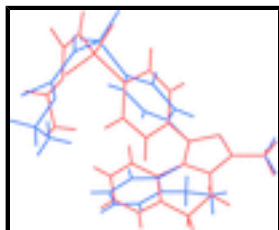
Fig. 2. Overlay diagram of the two independent organic molecules. The image in red contains the S1 atom.
