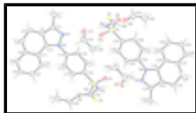
Fig. 1. The molecular structures of the two independent organic molecules and two independent ethanol molecules that comprise the crystallographic asymmetric unit in (I) showing the atom-labelling scheme and displacement ellipsoids at the 50% probability level.
