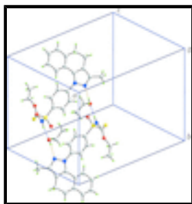
Fig. 3. Four-molecule aggregate in (I) mediated by O—H...N and N—H...O hydrogen bonding, shown as orange and blue dashed lines, respectively.
